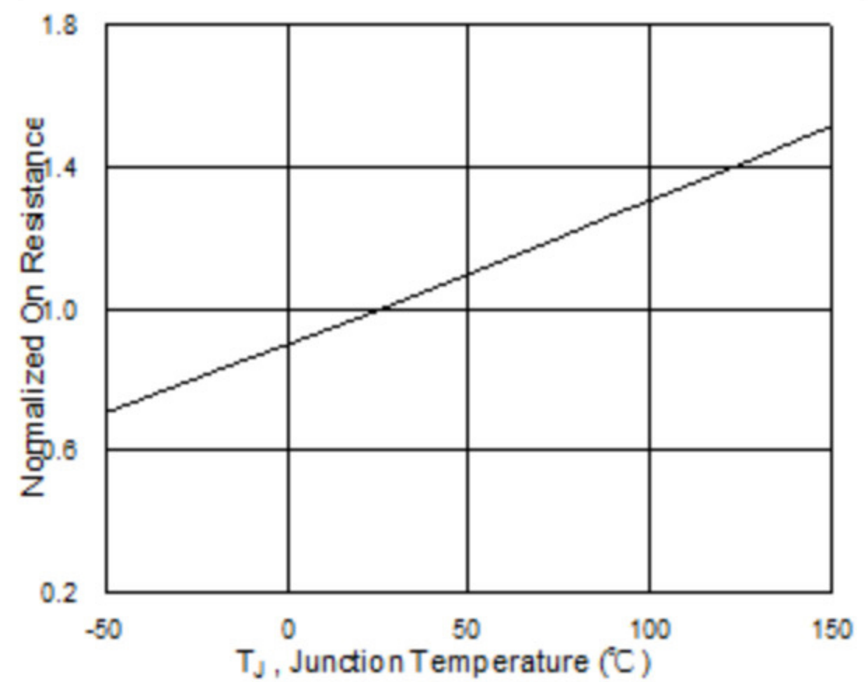
Fig.6 Normalized R_{DS(on)} vs. T_J
