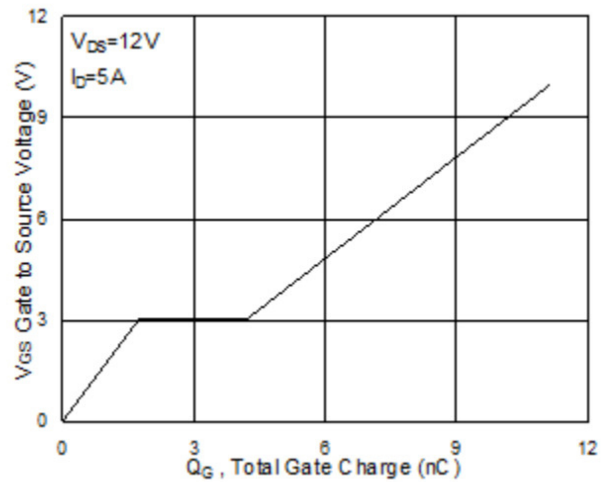
Fig.4 Gate-Charge Characteristics
