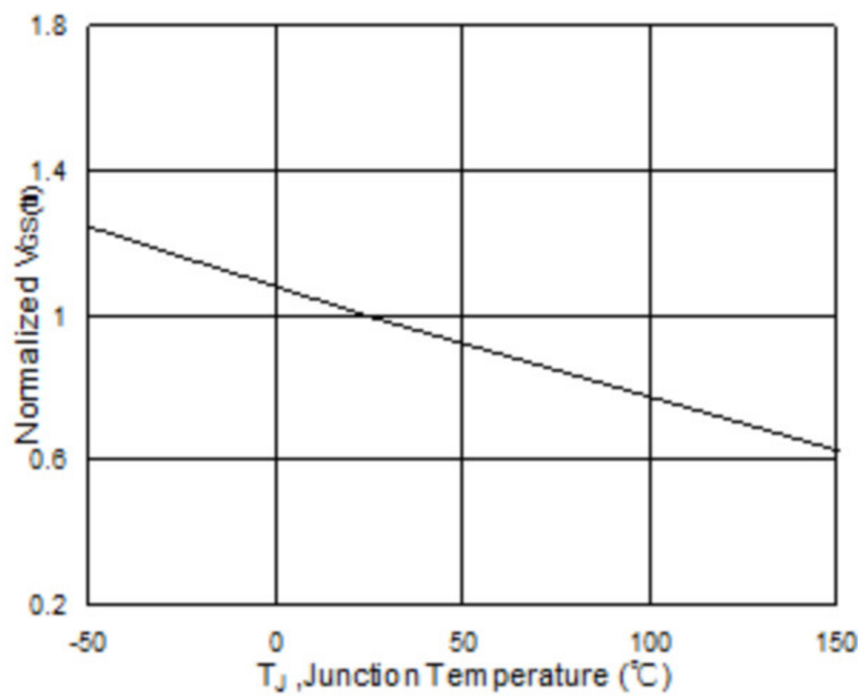
Fig.5 Normalized V_{GS(th)} vs. T_J
