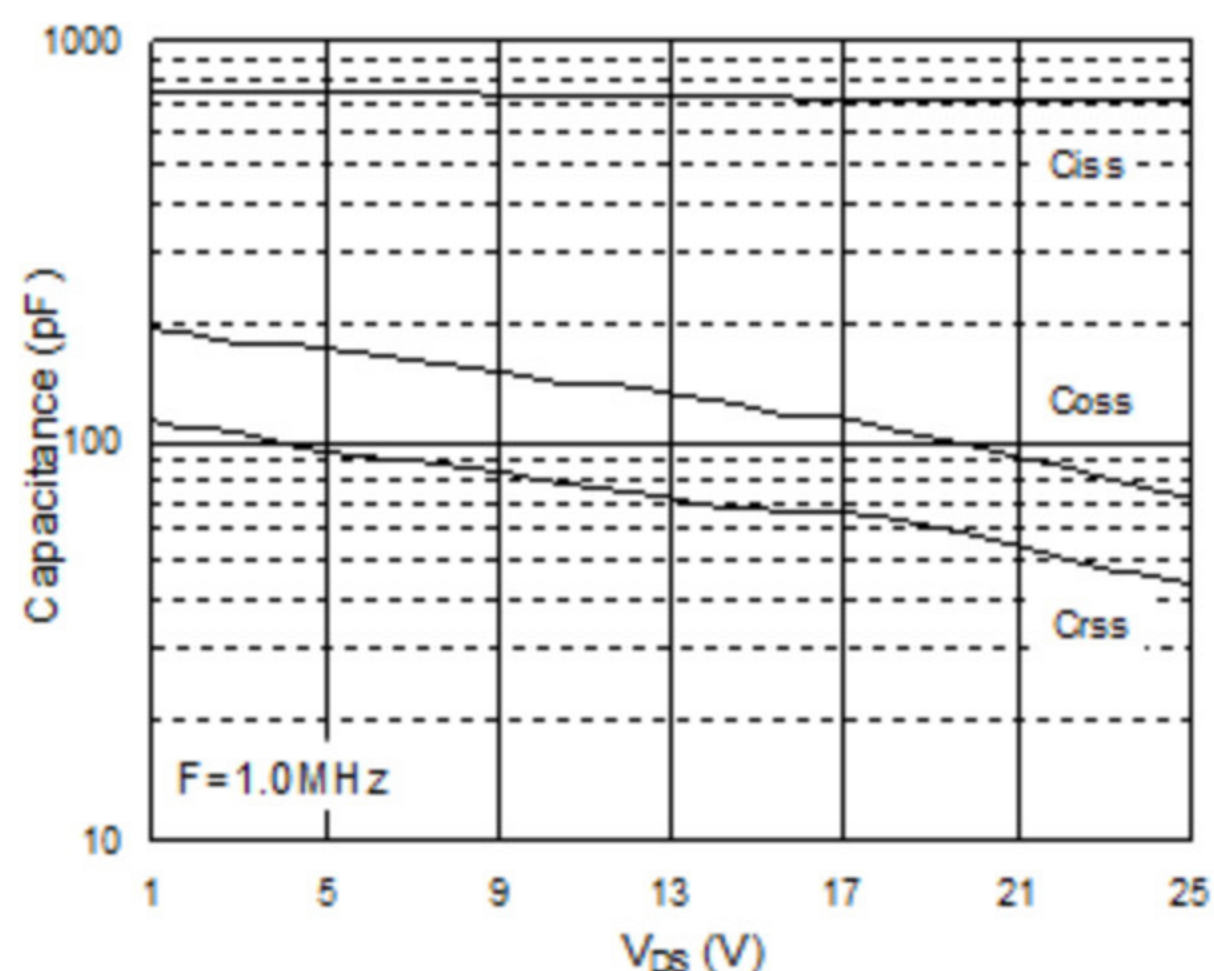
Fig.7 Capacitance
